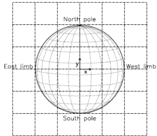
Figure A.1 Heliographic coordinate system. (figure 2 from Thompson, 2006)
