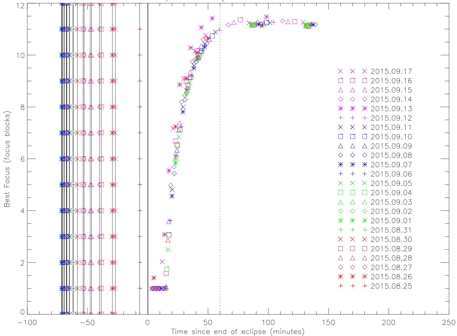
HMI Eclipse Recovery: 2015.08.25–2015.09.17
