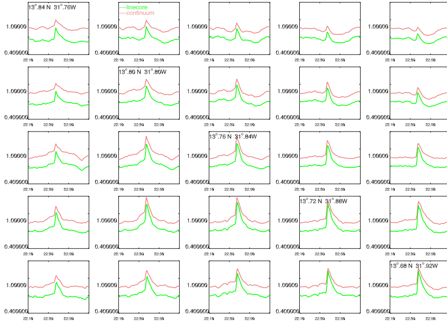
Figure 4. Mosaic of the time variation plots of the normalized continuum (red) and line-core (green) for a 5 \times 5 pixel section of the active region that produced the flare SOL2011-09-07T22:38:00. Each plot corresponds to a single pixel. The central pixel is located at 13^\circ.76\text{N} and 31^\circ.84\text{W} . The horizontal (time) axis spans 60 min. The continuum and line-core values have been normalized to a linear fit of the continuum intensity 15 minutes before and after the flare. Note, the linear fit was performed to de-trend the spacecraft motion from the continuum and line-core data. Figure 6 shows the selected section of the active region.
