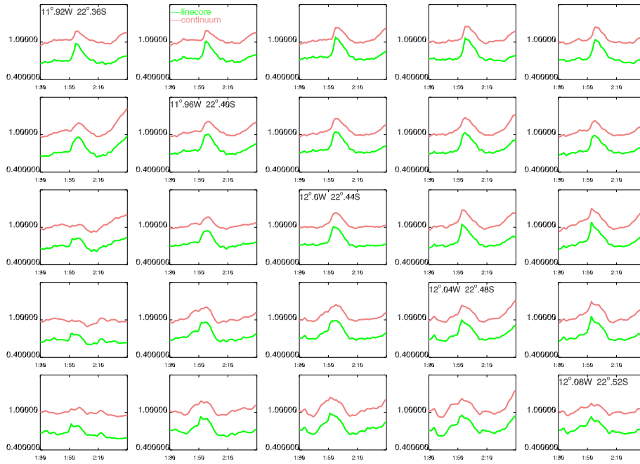
Figure 3. Mosaic of the time-variation plots of the normalized continuum (red) and line-core (green) intensity for a 5x5 pixel section of the active region of flare SOL2011-02-15T01:56:00. Each plot corresponds to a single pixel and the central pixel is located at 12^{\circ}.00W 22^{\circ}.44S . The horizontal axis spans a 60 min interval including the duration of the flare. The continuum and line-core values have been normalized by a linear fit of the continuum intensity 15 minutes before and after the flare. Note, the linear fit was performed to de-trend the effects of the spacecraft motion from the continuum and line-core data. Figure 2 shows the selected section of the active region.
