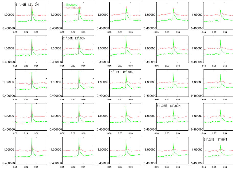
Figure 7. Mosaic of the time variation plots the normalized continuum (red) and line-core (green) intensity for a 5 \times 5 section of the active region that produced the flare SOL2011-09-24T09:40:00. Each plot corresponds to a single pixel and the central pixel is located at 61.32^\circ E and 12.04^\circ N. The horizontal (time) axis spans 120 min. The continuum and line-core values have been normalized to a linear fit of the continuum intensity 15 minutes before and after the flare. Note, the linear fit was performed to de-trend the effects of the spacecraft motion from the continuum and line-core data. Figure 8 shows the selected section of the active region .
